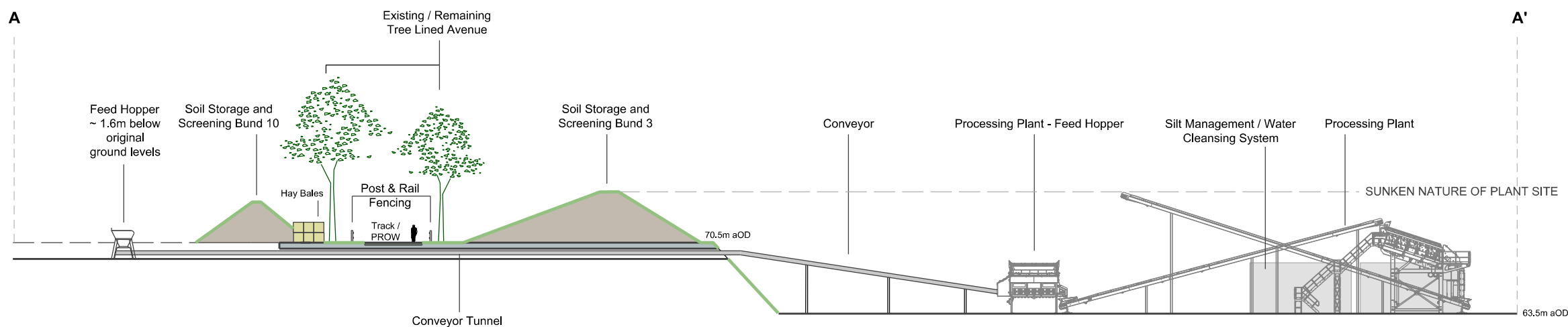
Section A-A' : Typical Section Along Conveyor Tunnel (1:500 @ A3)
