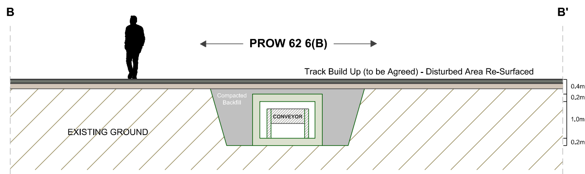
Section B-B' : Typical Cross Section Through Conveyor Tunnel (1:100 @ A3)
